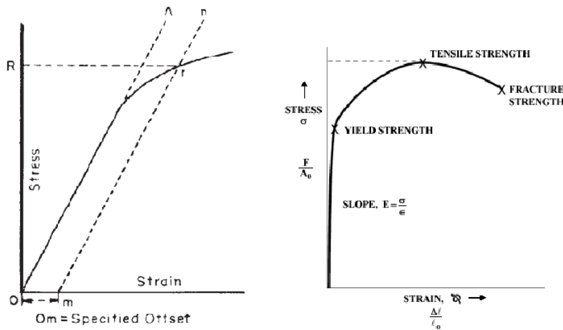
Figure 6. Definition of Yield Point
